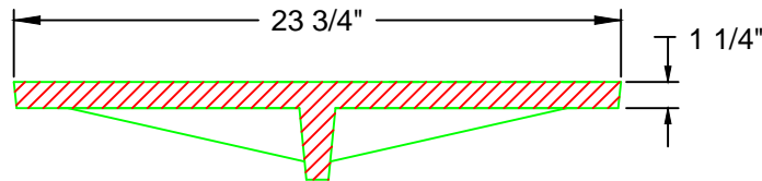
MANHOLE COVER TYPE J
