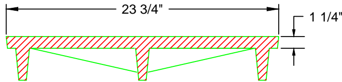
MANHOLE COVER TYPE CE
